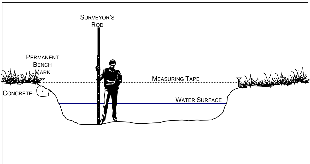
Figure 8: Technique for measuring the cross-sectional profile of a channel. Adapted from Rosgen (1996).
