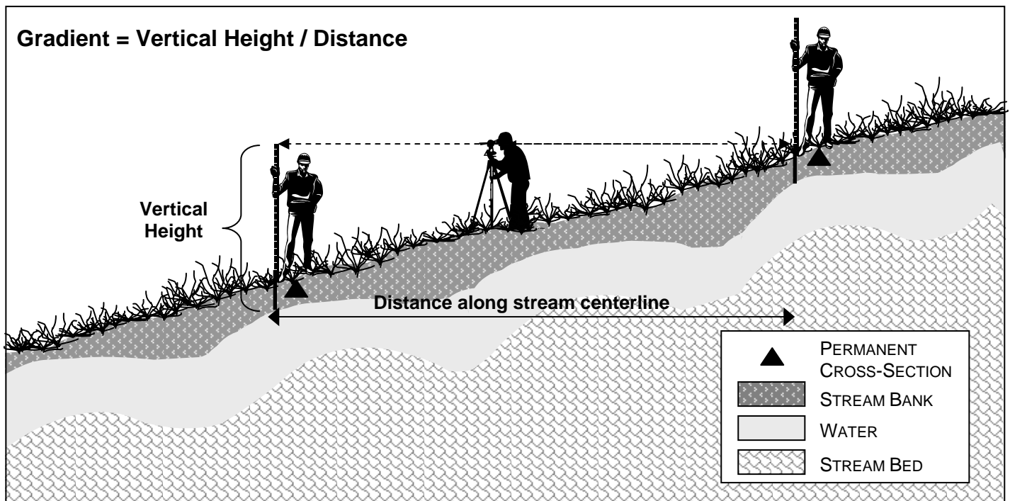
Figure 7: Longitudinal cross-sectional view of a stream, demonstrating the technique for measuring the longitudinal profile of a channel. The riffle-to-riffle gradient is an approximation of the average water surface slope of the reach. Adapted from Rosgen (1996).
