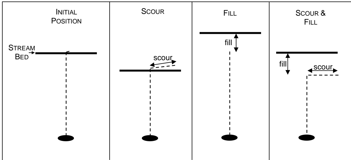
Figure 9: Use of scour chains to measure scour and fill depth of bed material. Arrows indicate points of measurement. Adapted from Bigelow (2003).
