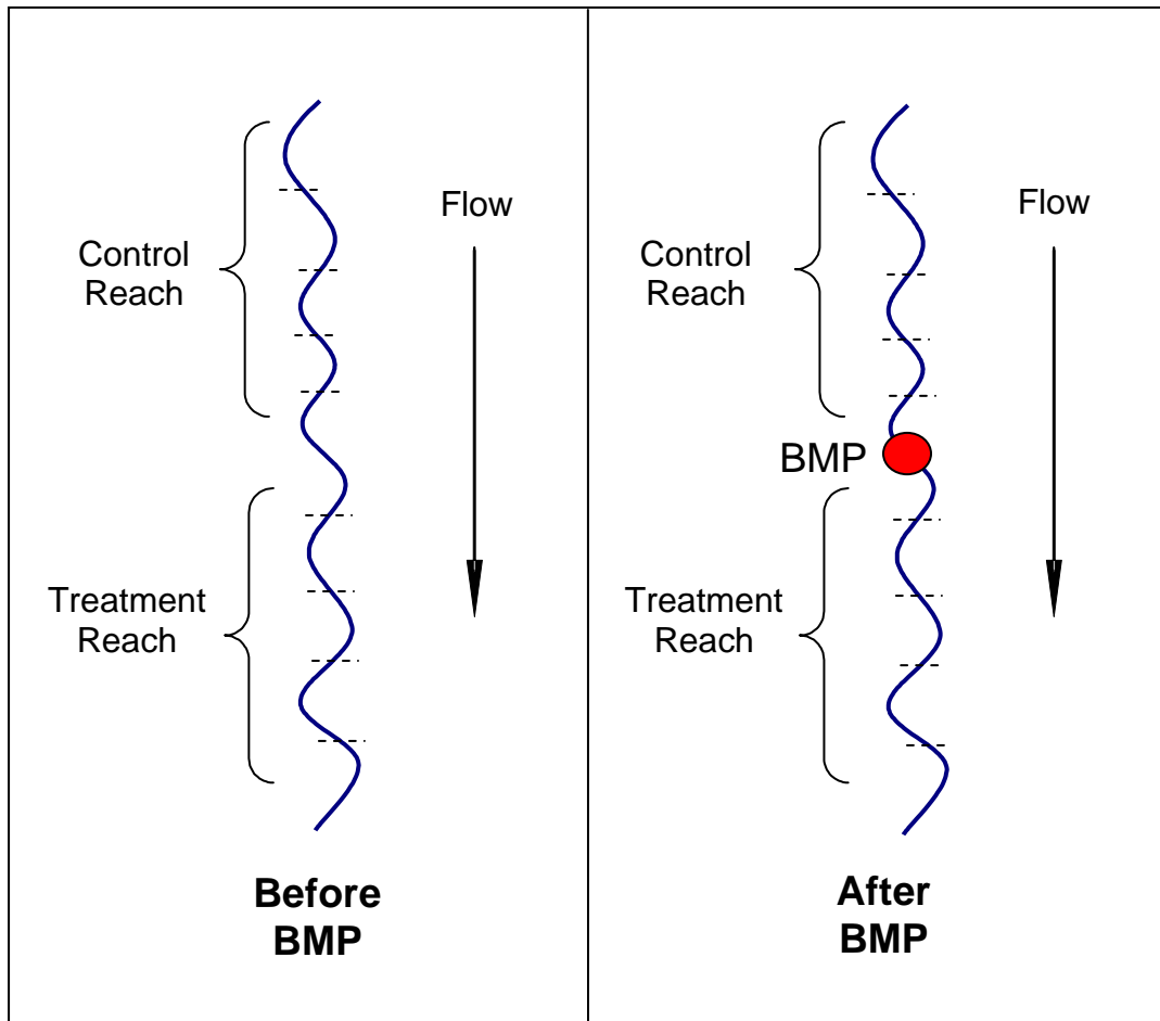
Figure 2: Before/After-Control/Impact (BACI) monitoring design, with upstream control and downstream treatment reaches. The dashed lines represent permanently established cross-sections.
