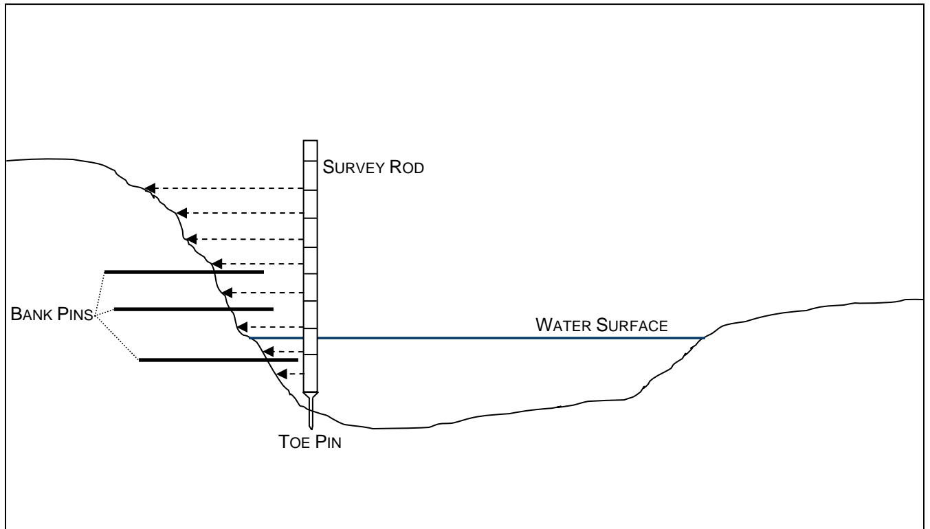
Figure 6: Example of bank pin placement and bank profile measurement. The arrows indicate measurement points for the bank profile. Modified from Rosgen (1996).
