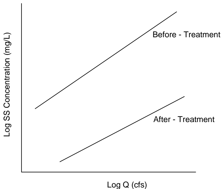
Figure 10: Hypothetical example of sediment rating curves, showing the relationship between suspended sediment (SS) and discharge (Q) for a treatment reach before and after BMP installation.
